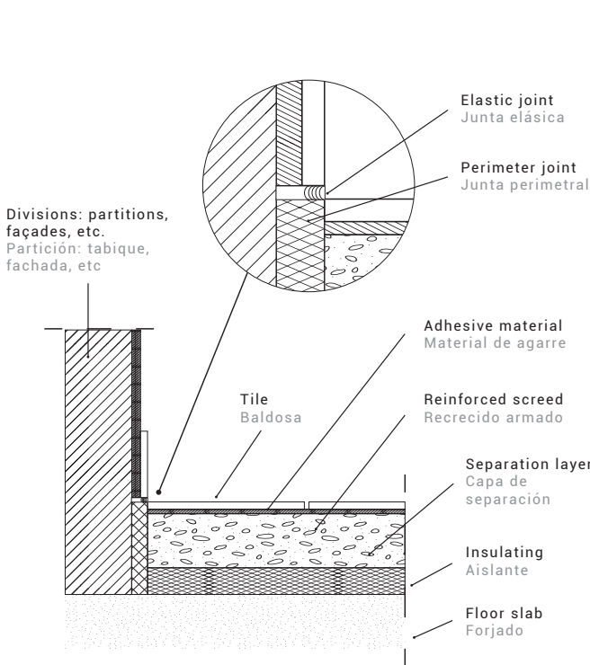
Detail of perimeter joint with sealant (UNE 138002:2017) Detalle de junta perimetral con sellante
